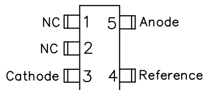
SOT-23-5 (Top View)
