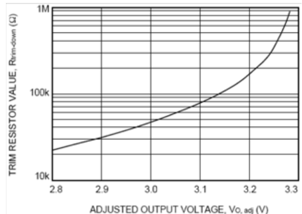
Figure 22. NH020F Rtrim-down Test Results .
