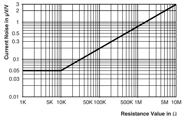
Current Noise
