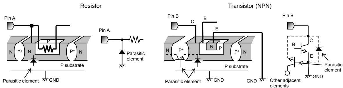
Figure.30 Example of IC structure
