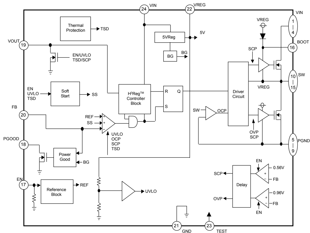
Figure.3 Block Diagram
