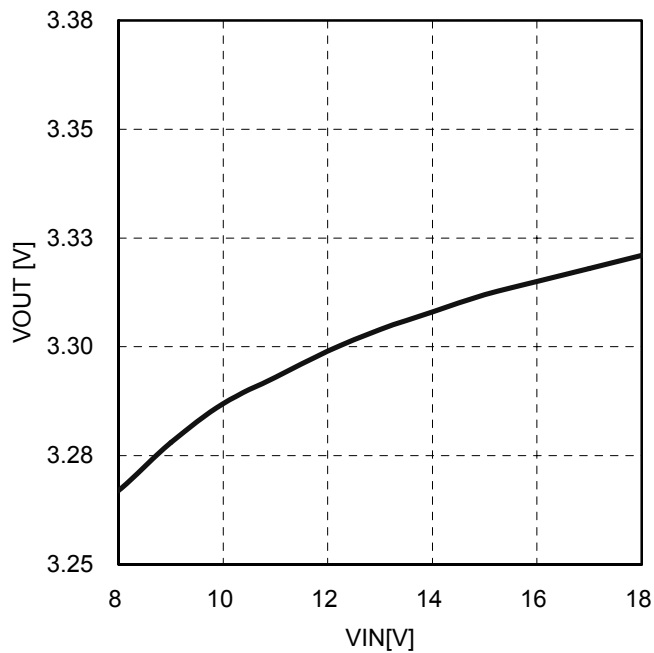
Figure.9 VOUT Line Regulation ( V_{OUT}=3.3\text{V} , L=2.2\mu\text{H} , I_{out}=0\text{A} )
