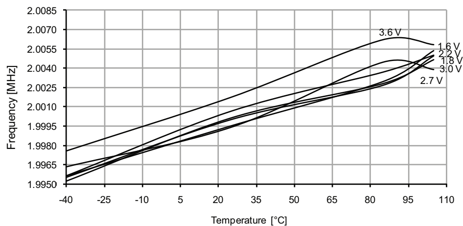
Figure 37-74. 2MHz internal oscillator frequency vs. temperature. DFLL enabled, from the 32.768kHz internal oscillator.
