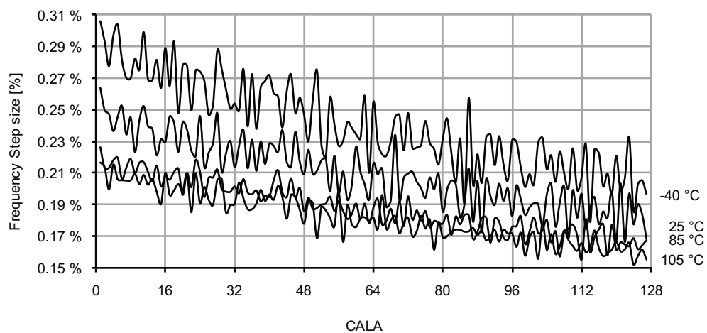
Figure 37-75. 2MHz internal oscillator CALA calibration step size. V_{CC} = 3V .
