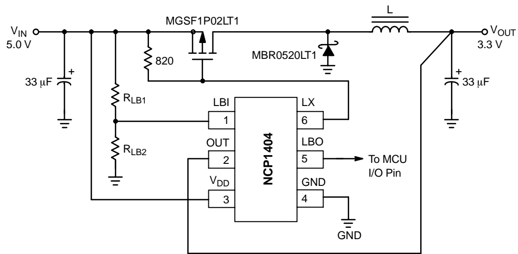
Figure 3. Step-down Application
