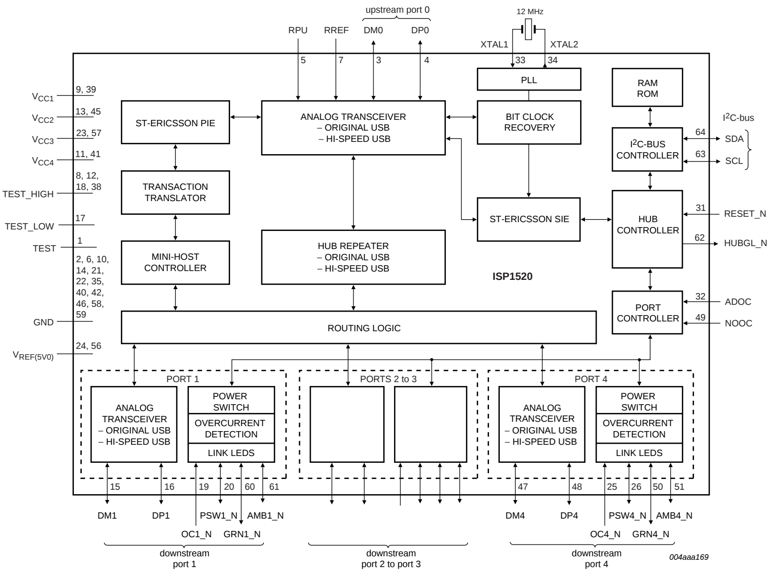
Fig 1. Block diagram
