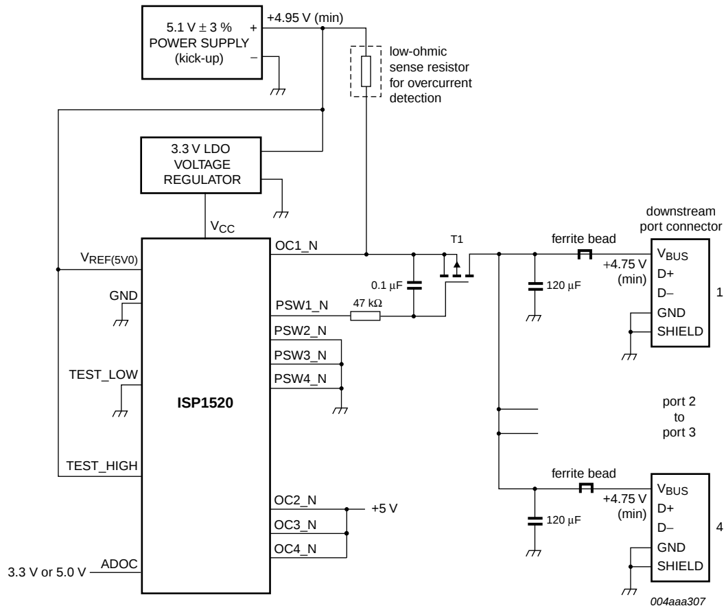
Fig 20. Self-powered hub; ganged port power switching; global overcurrent detection
