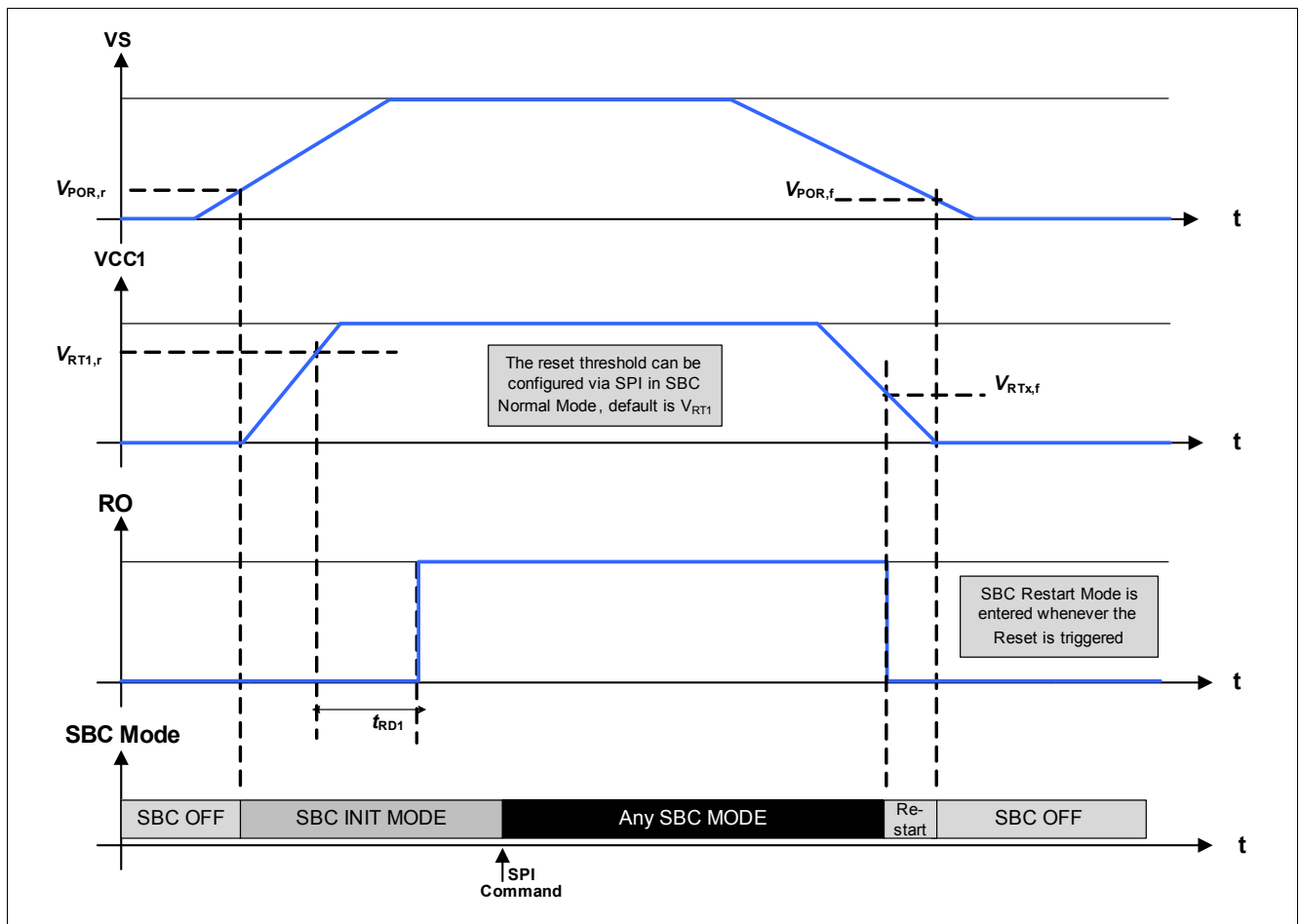
Figure 52 Ramp up / down example of Supply Voltage
