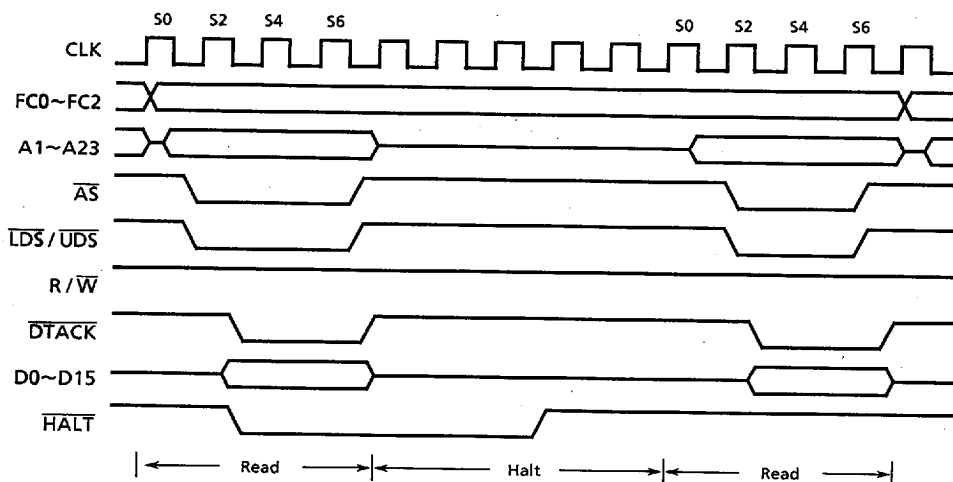
Figure 4.20 Halt Processor Timing Diagram
