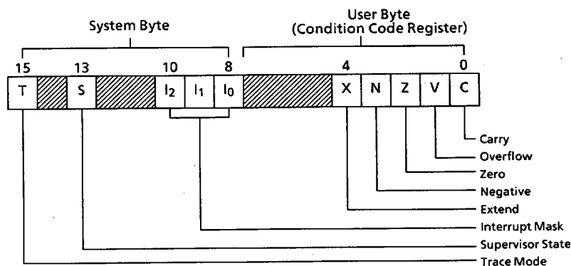
Figure 1.3 Status Register
