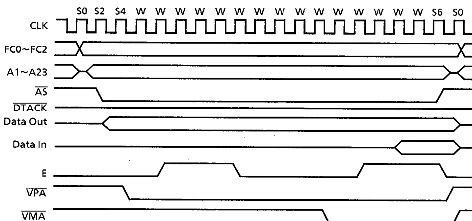
Figure 6.3 TMP68000 to 6800 Peripheral Timing – Worst Case
