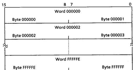
Figure 2.1 Word Organization in Memory
