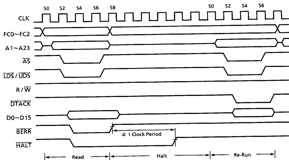
Figure 4.19 Re-Run Bus Cycle Timing Diagram
