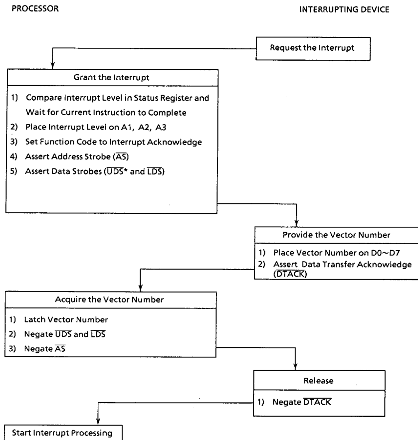
Figure 5.5 Vector Acquisition Flowchart
