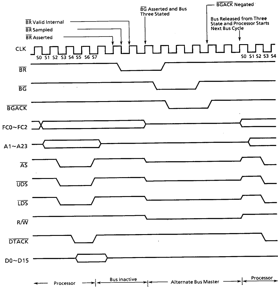
Figure 4.16 Bus Arbitration Timing Diagram - Bus Inactive
