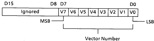
Figure5.2 Vector Number Format
