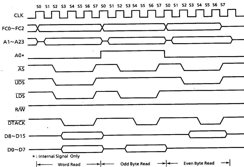
Figure 4.5 Word and Byte Read Cycle Timing Diagram
