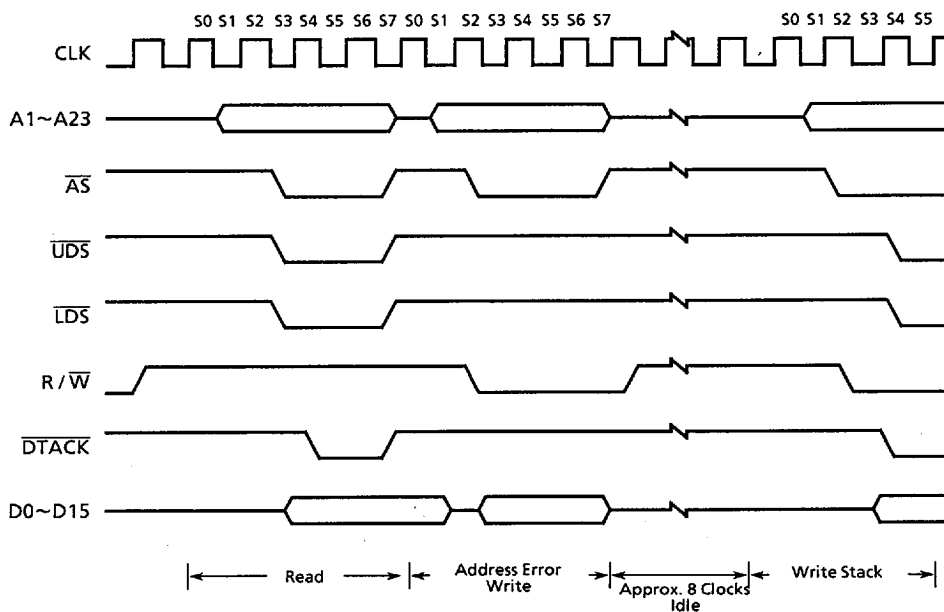
Figure 5.9 Address Error Timing Diagram
