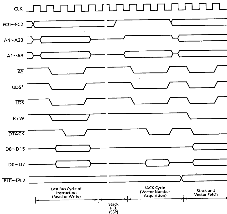
Figure5.6 Interrupt Acknowledge Cycle Timing Diagram
