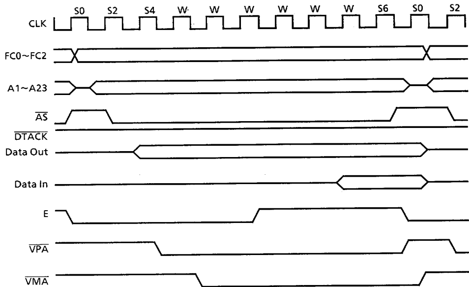
Figure 6.2 TMP68000 to 6800 Peripheral Timing – Best Case
