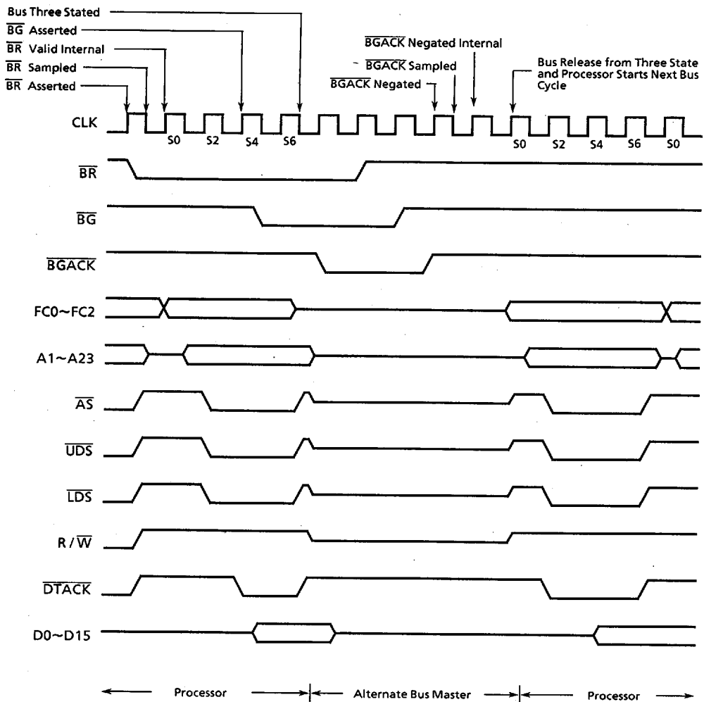
Figure 4.17 Bus Arbitration Timing Diagram - Special Case
