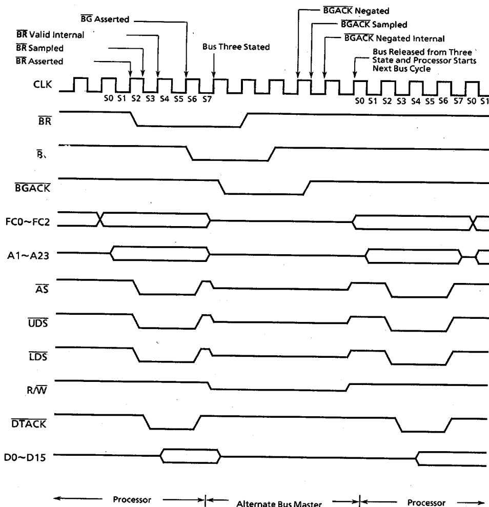
Figure 4.15 Bus Arbitration Timing Diagram – Processor Active
