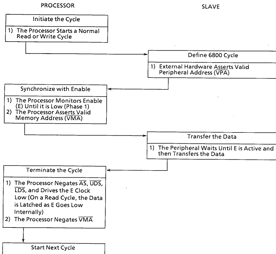
Figure 6.1 6800 Interfacing Flowchart
