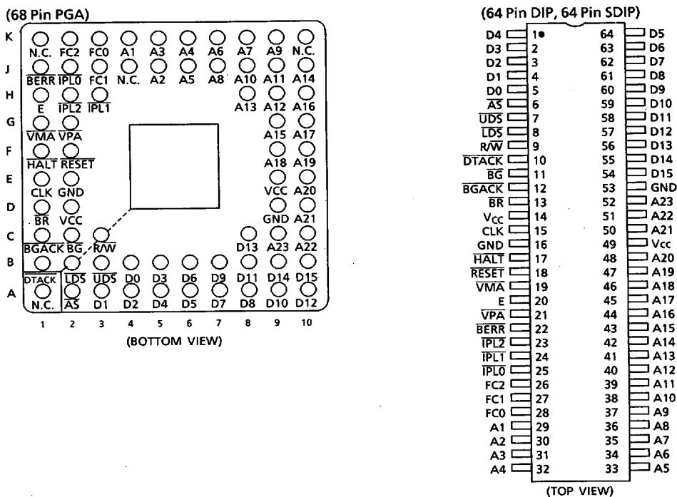
Figure 4.1 Input and Output Signals Pin Assignments (1/2)
