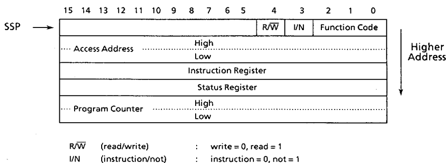
Figure 5.8 Exception Stack Order (Group 0)
