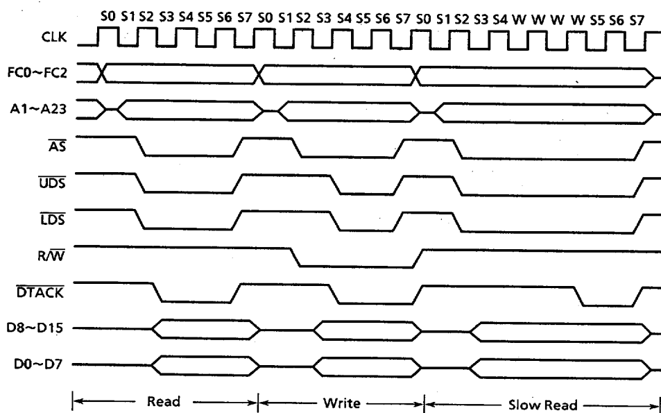
Figure 4.4 Read and Write Cycle Timing Diagram
