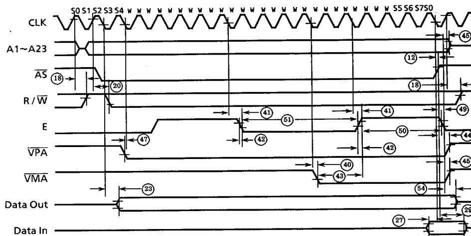
Figure 8.5 TMP68000 to 6800 Peripheral Timing Diagram – Best Case
