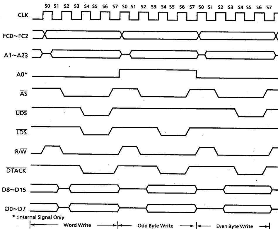
Figure 4.8 Word and Byte Write Cycle Timing Diagram
