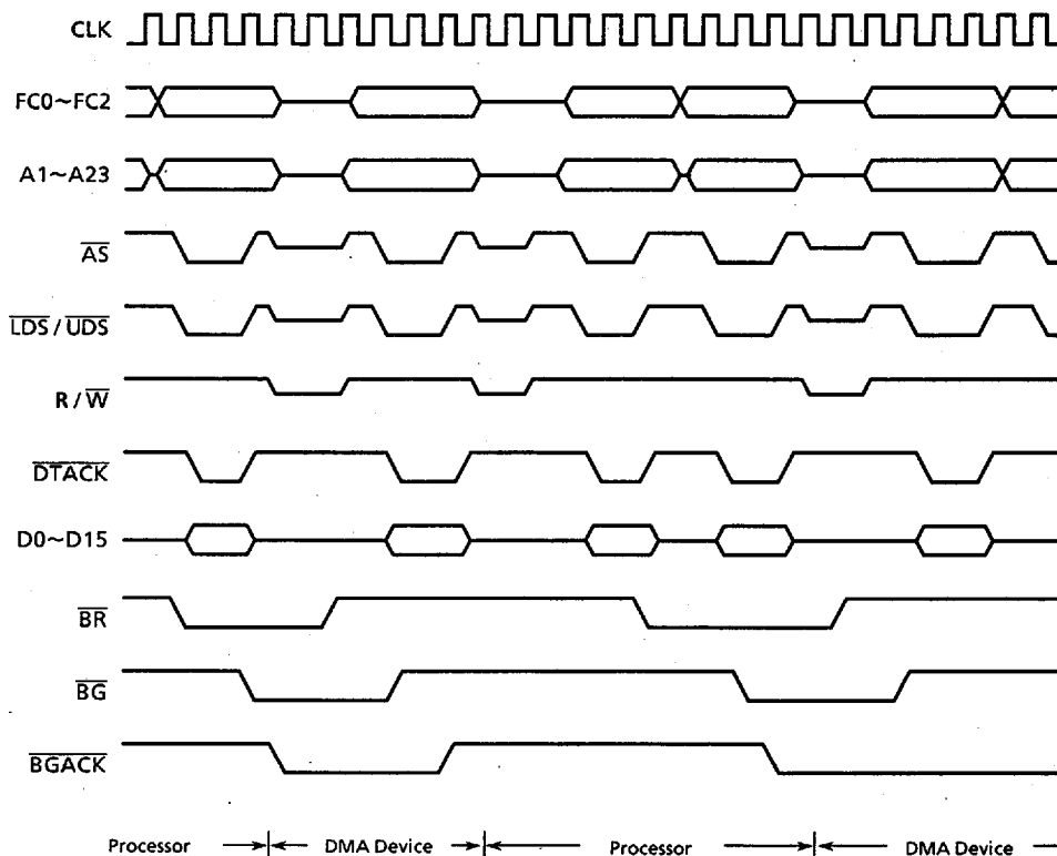
Figure 4.12 Bus Arbitration Cycle Timing Diagram
