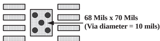
Figure 80. DGN PowerPAD PCB Etch and Via Pattern
