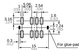
Suggested mounting pad (Top view)
