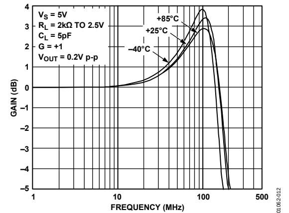
Figure 12. AD8054 Gain vs. Frequency vs. Temperature
