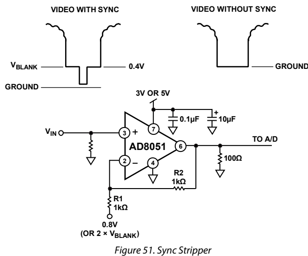
Figure 51. Sync Stripper
