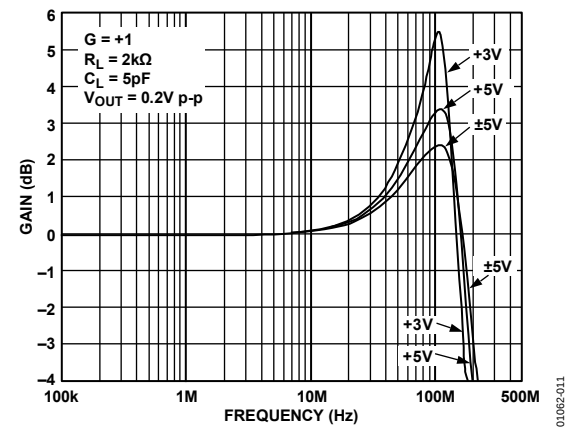
Figure 11. AD8054 Gain vs. Frequency vs. Supply
