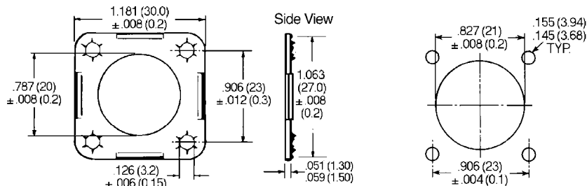
Mounting Dimensions
