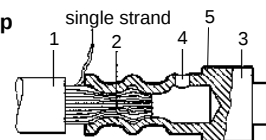
Incorrect Crimp
