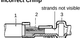
Incorrect Crimp
