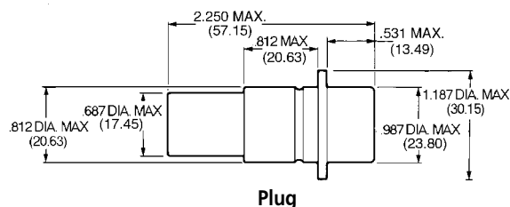
Plug
