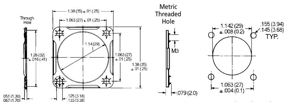
Mounting Dimensions
