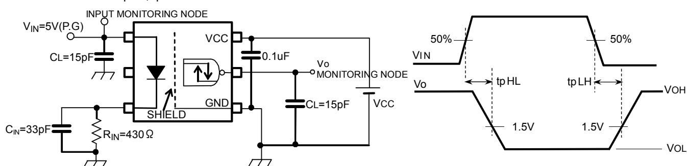
TEST CIRCUIT 2: t_{pLH} , t_{pHL}
