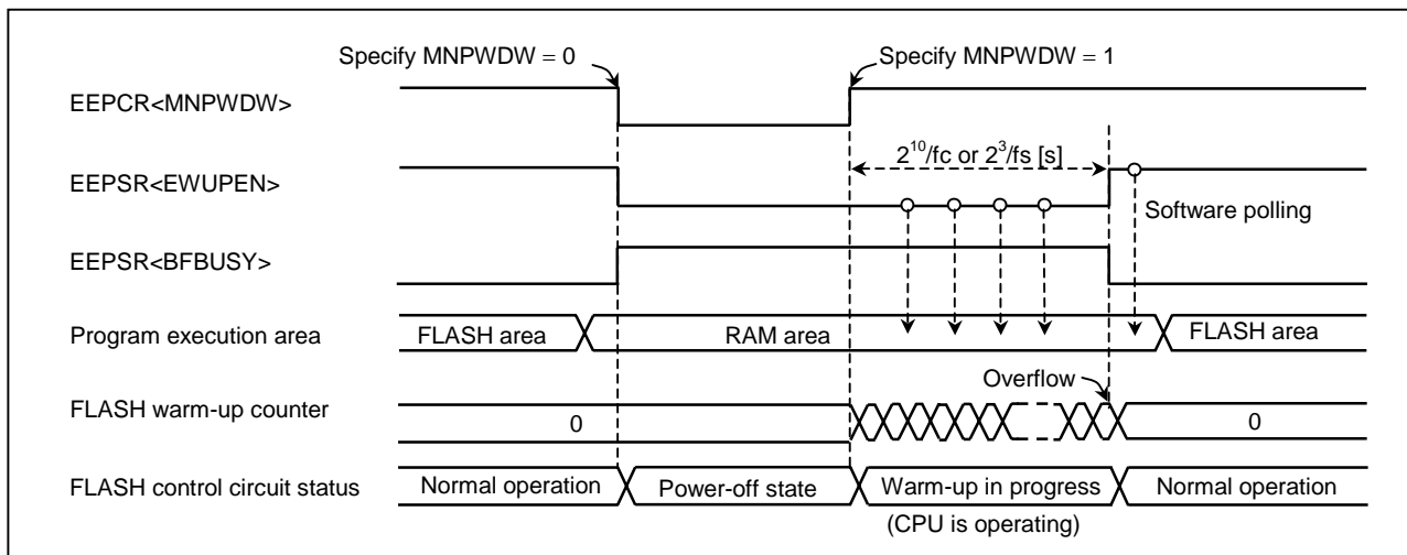
Figure 1.2.5 Software-based Power Control for the FLASH Control Circuit (EEPCCR<MNPWDW>)
