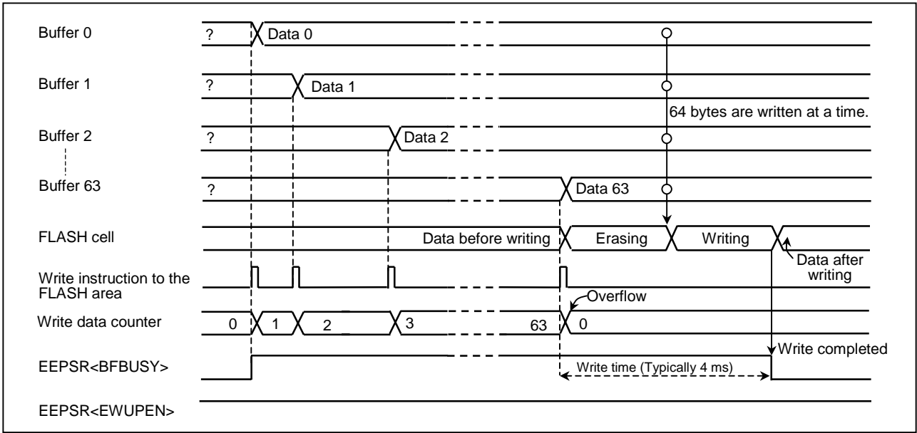
Figure 1.2.8 Write to the FLASH Area
