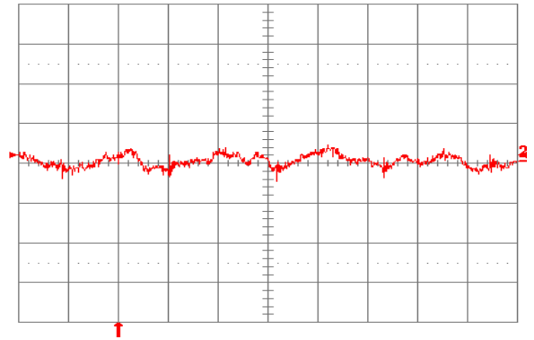
Fig. 2.5V.14: Input reflected-ripple current, i_e (10 mA/div.), measured through 10 \mu H at the source at full rated load current and V_{in} = 48 V. Refer to Fig. 2.5V.12 for test setup. Time scale: 1 \mu s/div.
