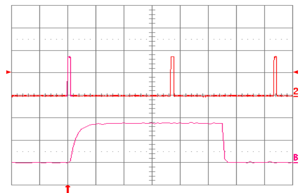
Fig. 3.3V.16: Load current (top trace, 20 \text{ A}/\text{div.} , 50 \text{ ms}/\text{div.} ) into a 10 \text{ m}\Omega short circuit during restart, at V_{in} = 48 \text{ V} . Bottom trace ( 20 \text{ A}/\text{div.} , 1 \text{ ms}/\text{div.} ) is an expansion of the on-time portion of the top trace.
