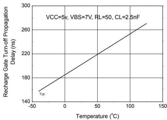
Figure 14. Recharge FET Turn-off Delay time
