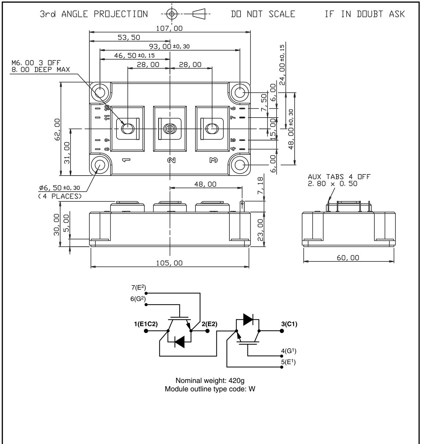
Fig. 11 Package details
