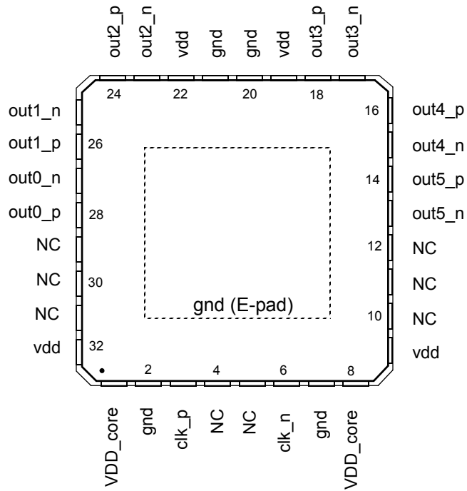
Figure 2 - Pin Connections
