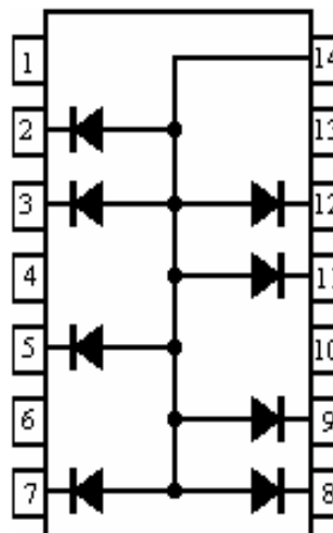
CIRCUIT CONFIGURATION
