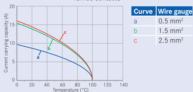
Turned contacts
