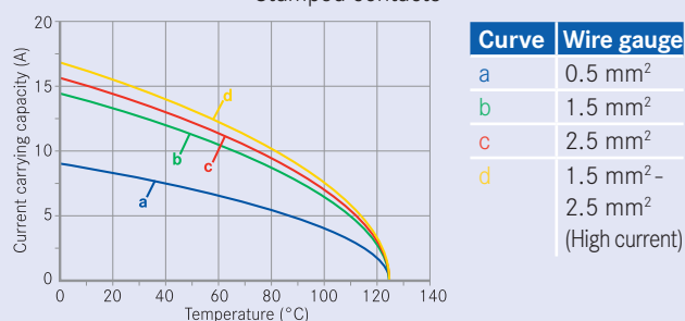
Stamped contacts
