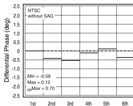
Figure 8. Differential Phase
