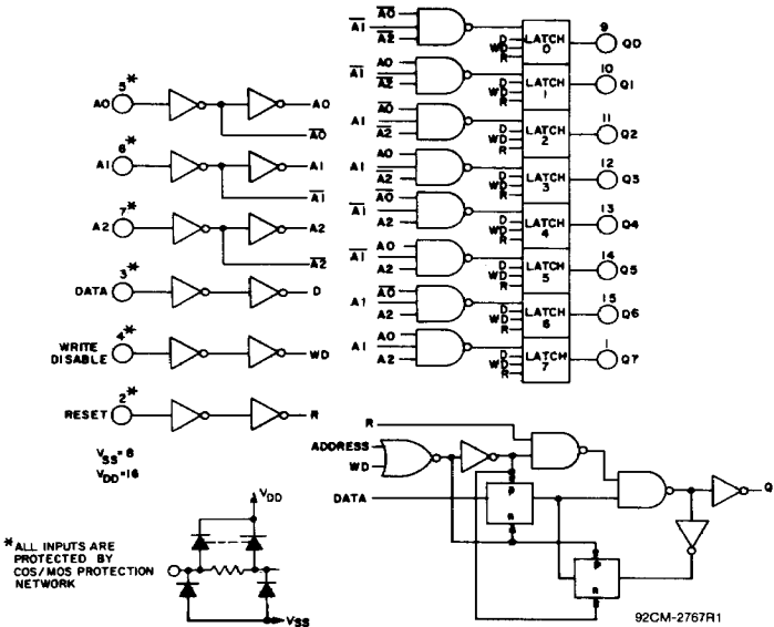
Fig. 1 - Logic diagram of CD4099B and detail of 1 of 8 latches.
