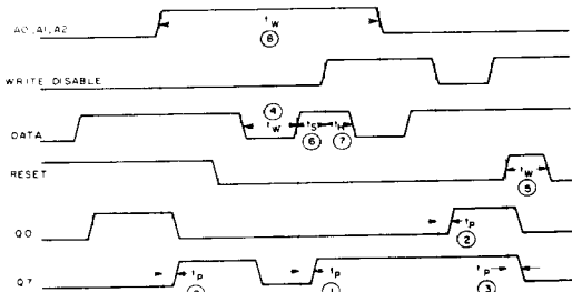
Fig. 15 — Master timing diagram.
