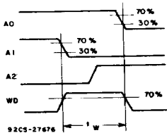
Fig. 3 - Definition of WRITE DISABLE ON time.
