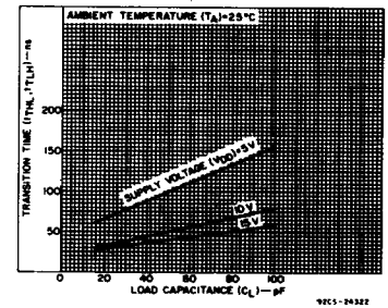
Fig. 9 — Typical transition time vs. load capacitance.
