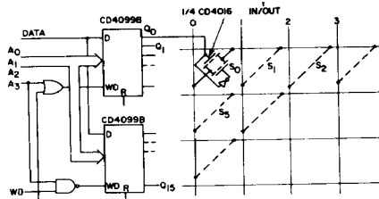
Fig. 16 — Multiple selection decoding — 4 x 4 crosspoint switch.
