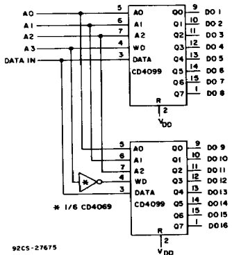
Fig. 14 — 1 of 16 decoder/demultiplexer.
