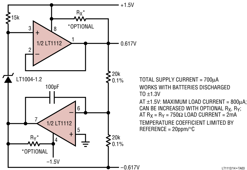
Dual Buffered \pm 0.617\text{V} Reference Powered by Two AA Batteries
