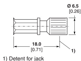
1) Detent for jack
