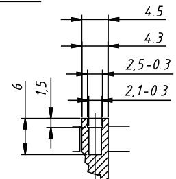
Detail Z
