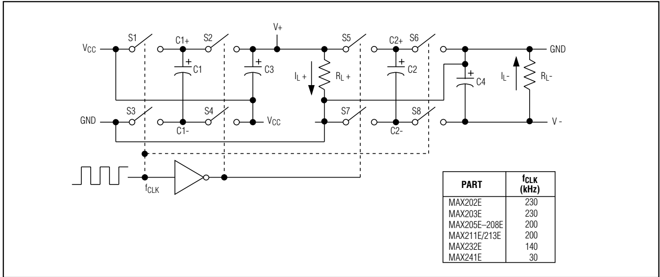
Figure 4. Charge-Pump Diagram
