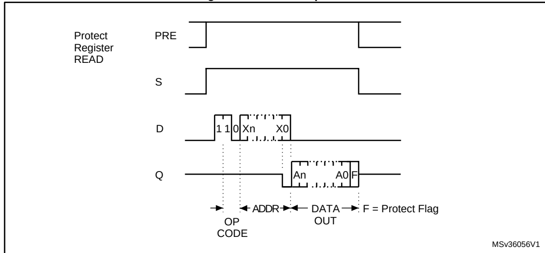
Figure 9: PREAD sequence
