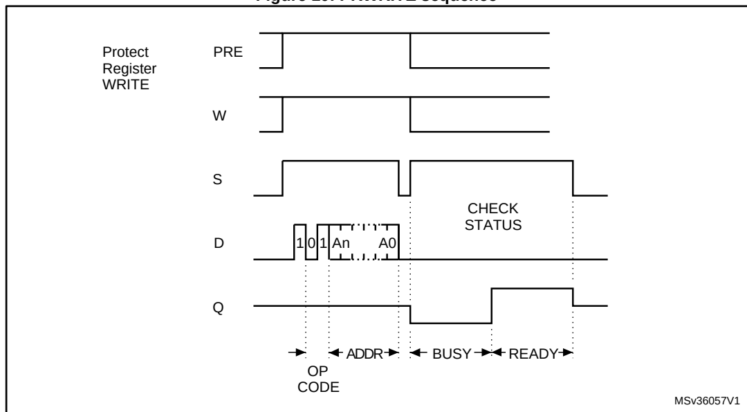
Figure 10: PRWRITE sequence
