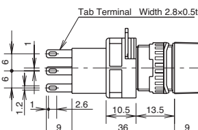
Solder/Tab Terminal
