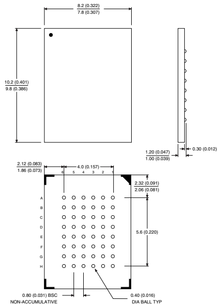
48U , 48-ball, Micro Ball Grid Array Package (μBGA) Dimensions in Millimeters
