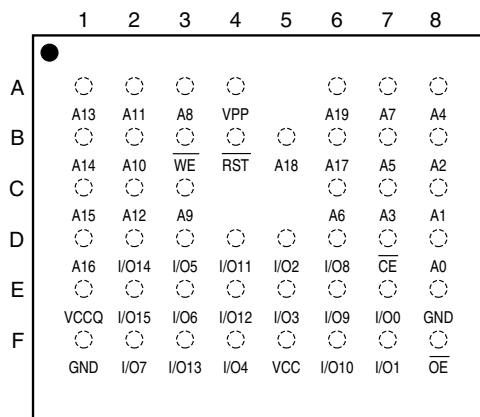
AT49BV1604(T) μBGA Top View (Ball Down)
