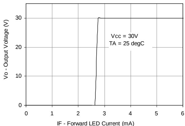
Figure 16: Transfer Characteristics
