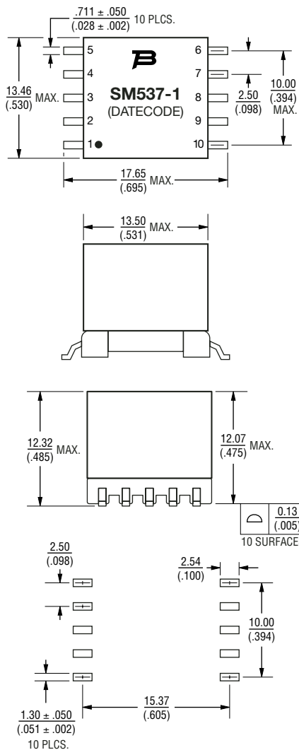
Recommended PAD layout
