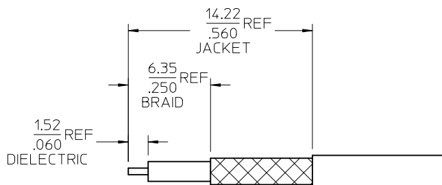
RECOMMENDED CABLE STRIP
