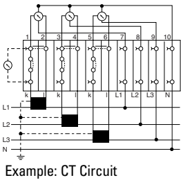
Example: CT Circuit
