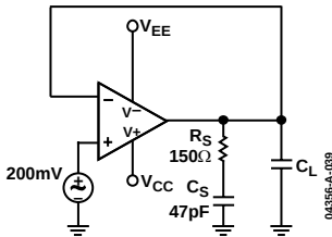
Figure 43. Snubber Network
