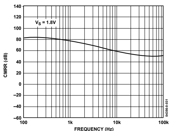
Figure 34. Common-Mode Rejection Ratio vs. Frequency
