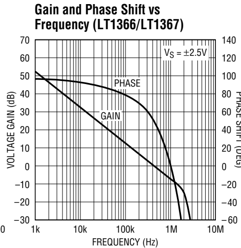
LT1366 TPC14
