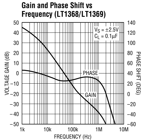
LT1366 TPC15
