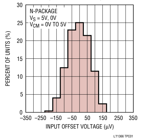
\Delta V_{OS} -Shift Between PNP and NPN Stages (LT1366/LT1368)
