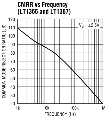
LT1366 TPC16
