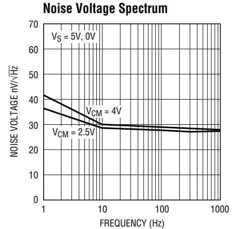
LT1366 TPC12
