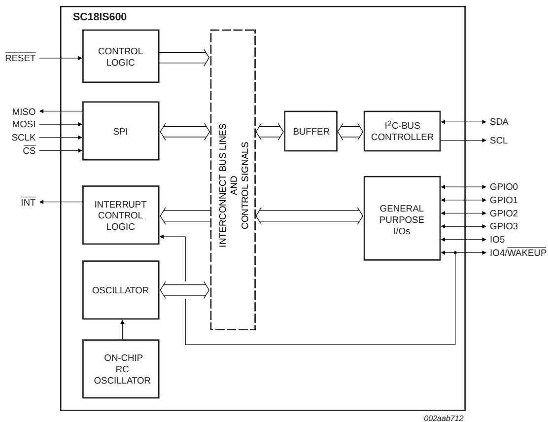
Fig 1. Block diagram of SC18IS600
