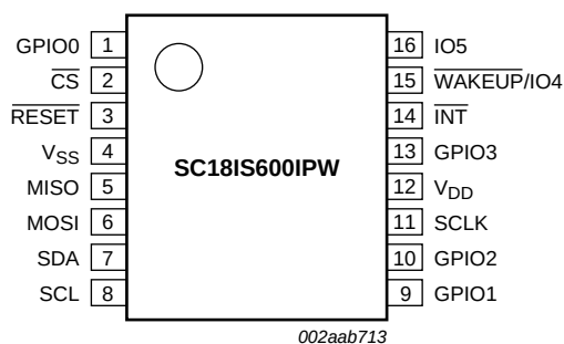
Fig 2. SC18IS600 pin configuration for TSSOP16
