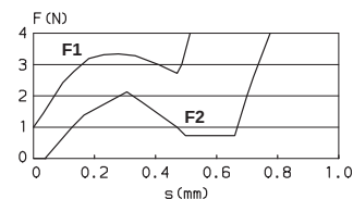
FORCE/TRAVEL DIAGRAM
