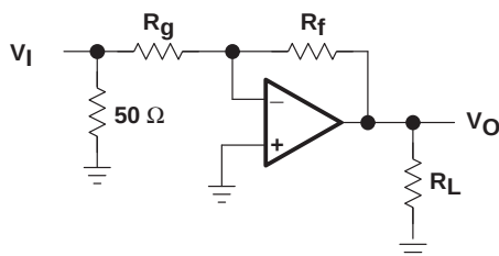
Figure 4. Step Response Test Circuit
