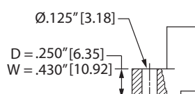
FLUSH MOUNTING (D, W)
