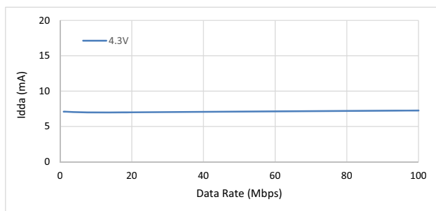
Figure 10. Si88620 Typical V_{DDA} Supply Current vs. Data Rate Using VREGA (4.3 V)
