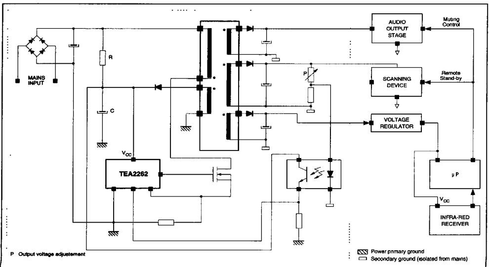
Figure 2 : Secondary Regulation (with optocoupler)
