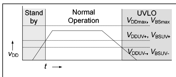
Figure 4: Operating states
