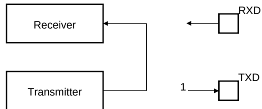
Figure 21-41. Local Loopback Mode Configuration
