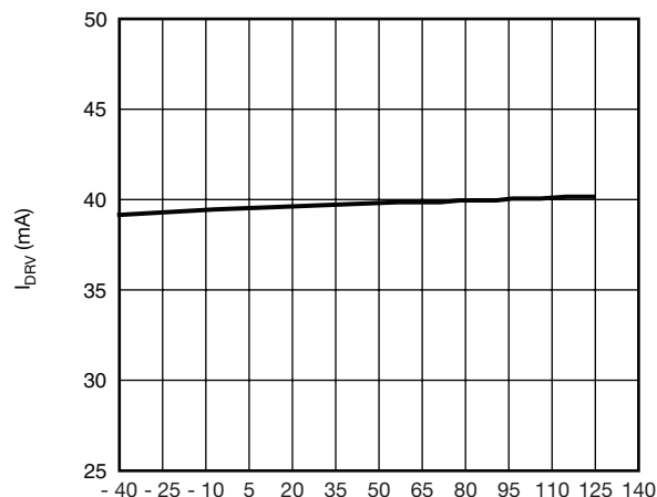
Temperature (°C) I DRV (mA) vs. Temperature at Frequency = 1 MHz D = 10\% , V_{CIN} = V_{DRV} = 5\text{ V}
