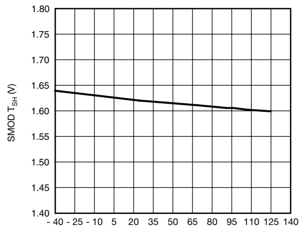
Temperature (°C) SMOD Rising Threshold (V) vs. Temperature (°C) V_{CIN} = V_{DRV} = 5\text{ V}
