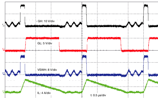
Switching Waveforms with SMOD Enabled V_{IN} = 12\text{ V} , V_{OUT} = 1.2\text{ V} , f_S = 500\text{ kHz} , I_{OUT} = 0\text{ A}
