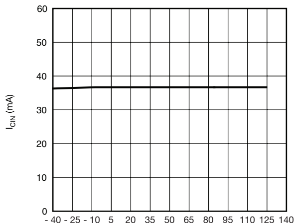
Temperature (°C) I CIN + I DRV (mA) vs. Temperature at Frequency = 1 MHz D = 10\% , V_{CIN} = V_{DRV} = 5\text{ V}
