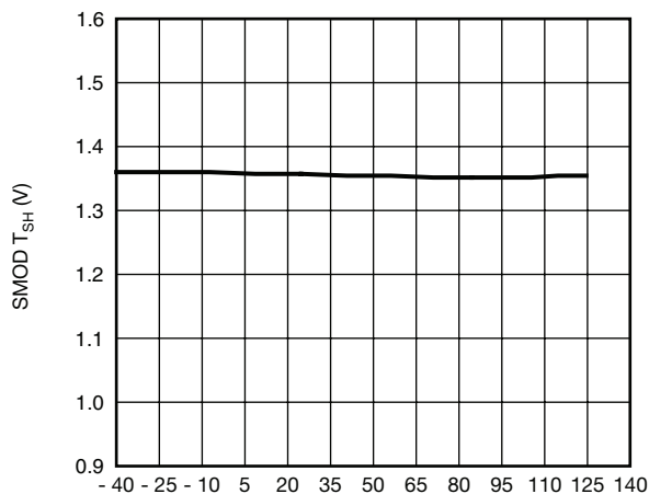
Temperature (°C) SMOD Falling Threshold (V) vs. Temperature (°C) V_{CIN} = V_{DRV} = 5\text{ V}
