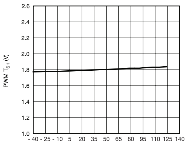
Temperature (°C) PWM Falling Tristate (V) vs. Temperature (°C) V_{CIN} = V_{DRV} = 5\text{ V}
