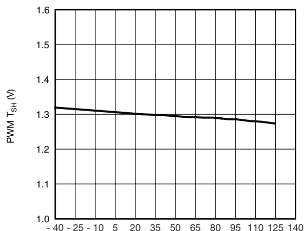
Temperature (°C) PWM Rising Tristate Threshold (V) vs. Temperature (°C) V_{CIN} = V_{DRV} = 5\text{ V}
