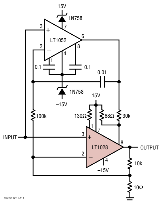
Chopper-Stabilized Amplifier
