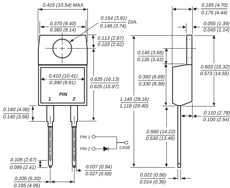
TO-220AC (GUR5H60)
