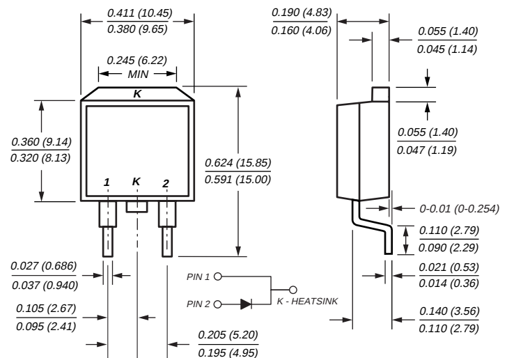
TO-263AB (GURB5H60)
