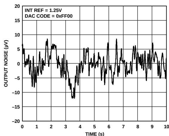
Figure 40. 0.1 Hz to 10 Hz Output Noise Plot, Internal Reference
