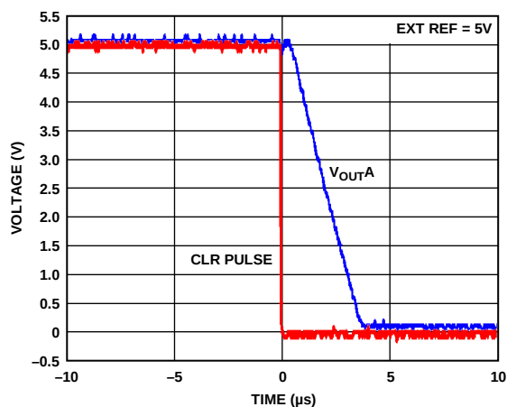
Figure 44. Hardware \overline{CLR}
