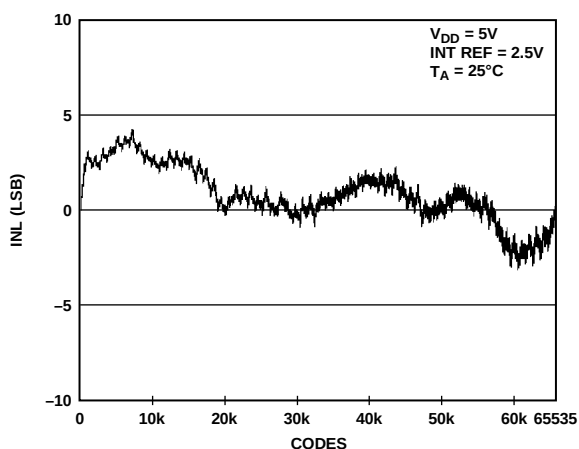
Figure 10. INL AD5669R-2—Internal Reference
