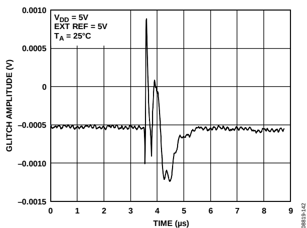
Figure 36. Analog Crosstalk
