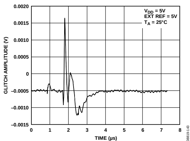
Figure 37. DAC-to-DAC Crosstalk
