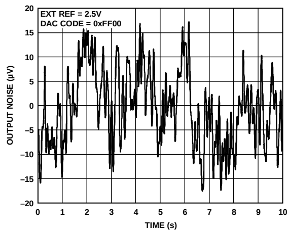
Figure 39. 0.1 Hz to 10 Hz Output Noise Plot, Internal Reference
