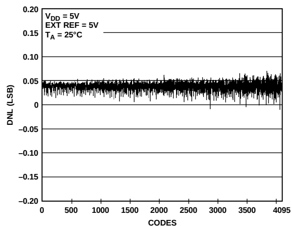
Figure 9. DNL AD5629R—External Reference
