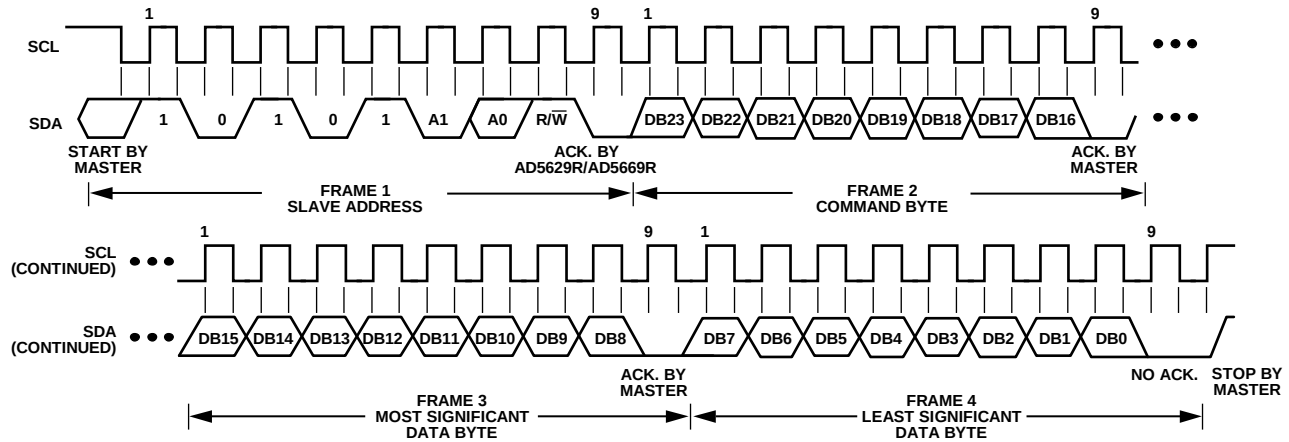
Figure 52. I²C Read Operation
