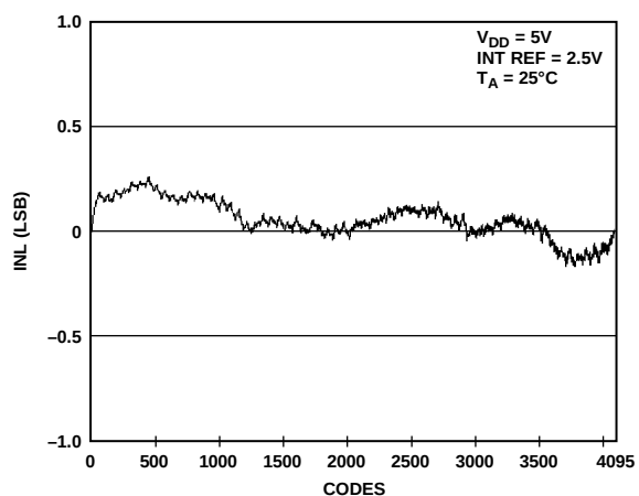
Figure 11. INL AD5629R-2—Internal Reference
