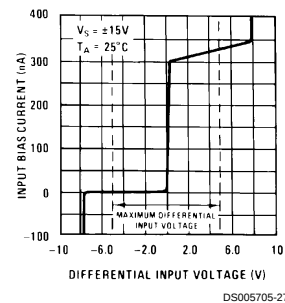
Input Characteristics
