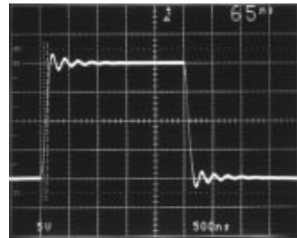
Figure 6. Large-Signal Response, C_L = 10,000 pF
